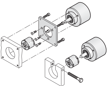
Clamping flange
